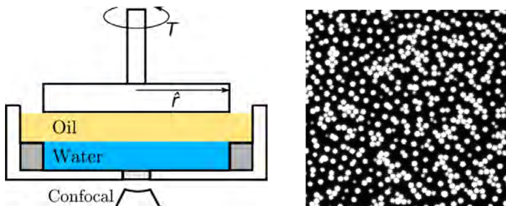
Figure 1: (left) Schematic of set-up for contactless interfacial rheology. (right) Confocal micrograph of micron-sized interfacial particles.
