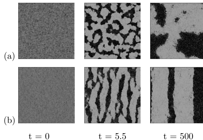
Figure 1: Phase separation after quenching a system of self-propelled particles into the two-phase region. Snapshots of the system at various times after the quench, for the alignment field strengths (a) \tilde{B} = 0 at the critical packing fraction \phi = 0.60 at Pe = 138 and (b) \tilde{B} = 2 at \phi = 0.63 at Pe = 221 . The time t is given in MD time and the system size is 512\sigma \times 512\sigma .
