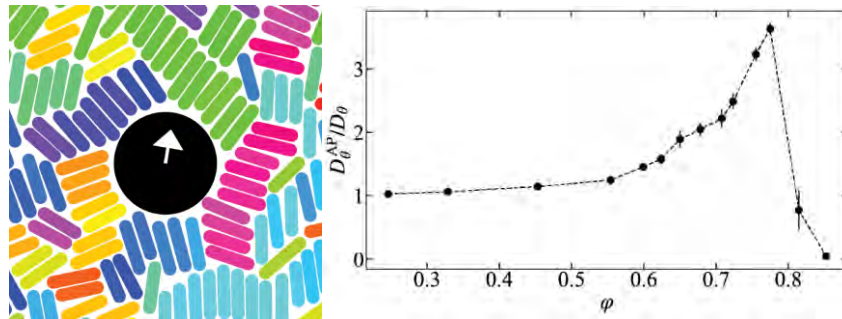
Figure 1: (left) Snapshot of an active probe in our simulation study; colors indicate rod orientation. (right) The associated ERD as a function of rod area fraction.
